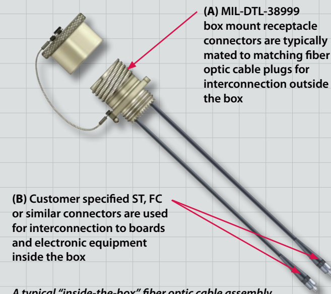
A typical "inside-the-box" fiber optic cable assembly. Cables of this type are now available as a standard short-lead catalog product from Glenair.
