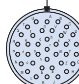
Shell Size 25 Arrangement 37
