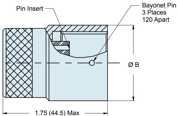
07 Receptacle Adapter U.S. PATENT NO. 5,960,137
