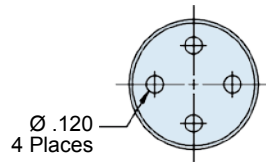
HOLE PATTERN SHELL SIZE 13 SHOWN
