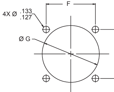
Recommended Panel Cut-Out for Wall Mount Receptacles
