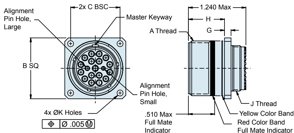
H7 - Wall Mount Receptacle with Standard Holes
