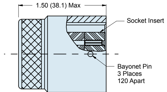
07 Receptacle Adapter U.S. PATENT NO. 5,960,137
