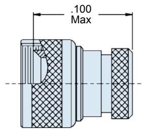
SHRINK BOOT ADAPTER (STD)
